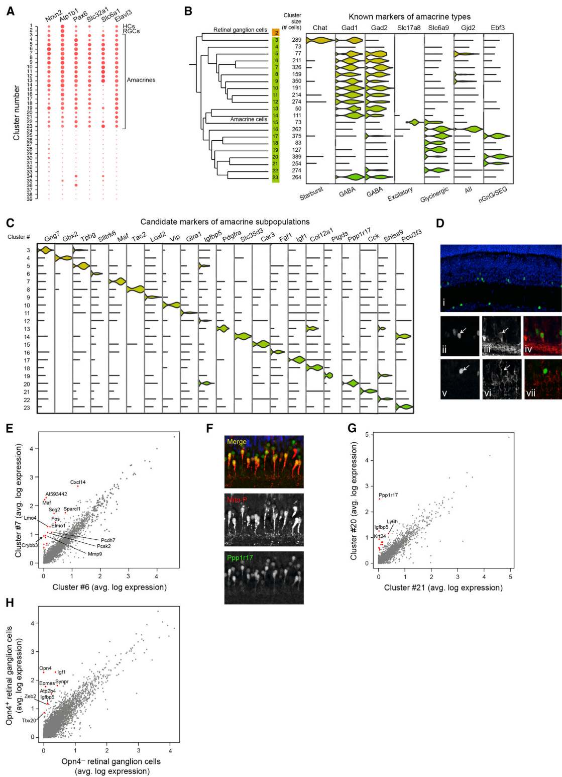
Figure 6. Finer-Scale Expression Distinctions among Amacrine Cells, Cones, and Retinal Ganglion Cells (A) Pan-amacrine markers. The expression levels of the six genes identified ( Nrxn2 , Atp1b1 , Pax6 , Slc32a1 , Slc6a1 , Elavl3 ) are represented as dot plots across all 39 clusters; larger dots indicate broader expression within the cluster; deeper red denotes a higher expression level.
